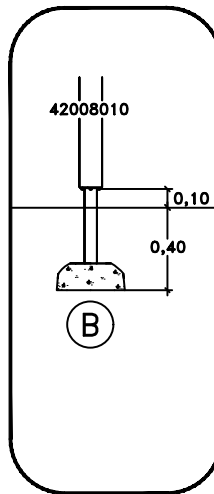
Sunken Foundation
